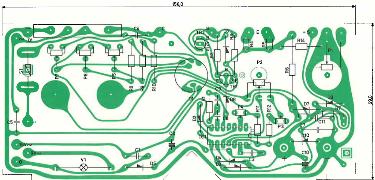
Fig. 15. Komponentplacering Component Location
